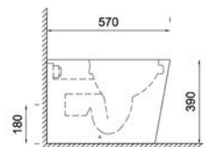
SECTION VIEW
