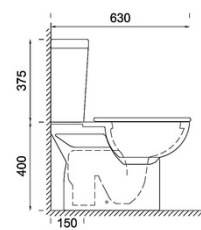
SECTION VIEW
