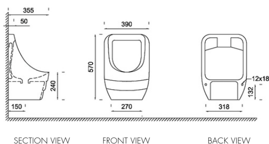
Chelsey ST2201-AB ADA Anti-Bacterial HPKV Waterless Urinal L 390 x W 355 x H 570 mm WELS: ✓✓✓
