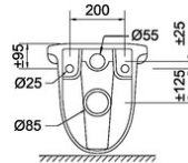
BACK VIEW
