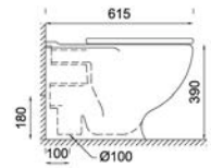
SECTION VIEW
