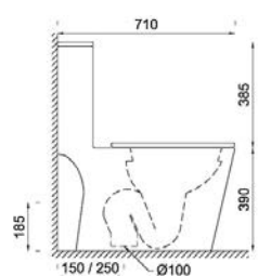
SECTION VIEW
