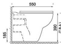
SECTION VIEW
