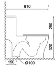
SECTION VIEW
