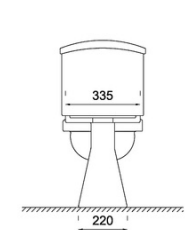
BACK VIEW
