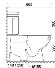
SECTION VIEW
