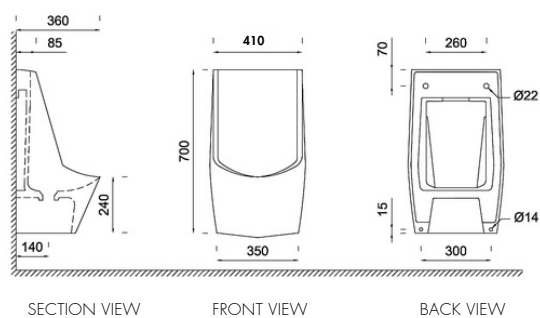
Capparis ST2205-AB Anti-Bacterial HPKV Waterless Urinal L 410 x W 360 x H 700 mm WELS: ✓✓✓
