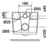
BACK VIEW
