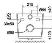
BACK VIEW
