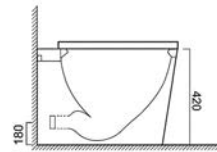
SECTION VIEW
