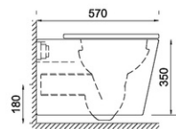
SECTION VIEW
