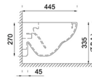
SECTION VIEW
