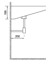
SECTION VIEW
