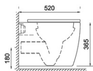
SECTION VIEW
