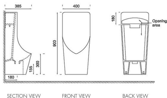
Mimosa ST2215-AB Anti-Bacterial HPKV Waterless Urinal L 400 x W 385 x H 900 mm WELS: ✓✓✓
