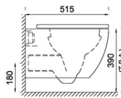
SECTION VIEW
