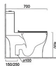
SECTION VIEW
